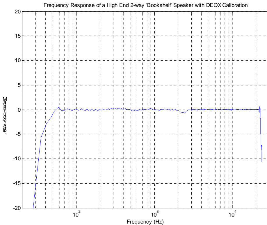
A typical frequency response of a 2-way speaker system after DEQX Calibrated™ 'speaker' correction showing woofer and tweeter combined
