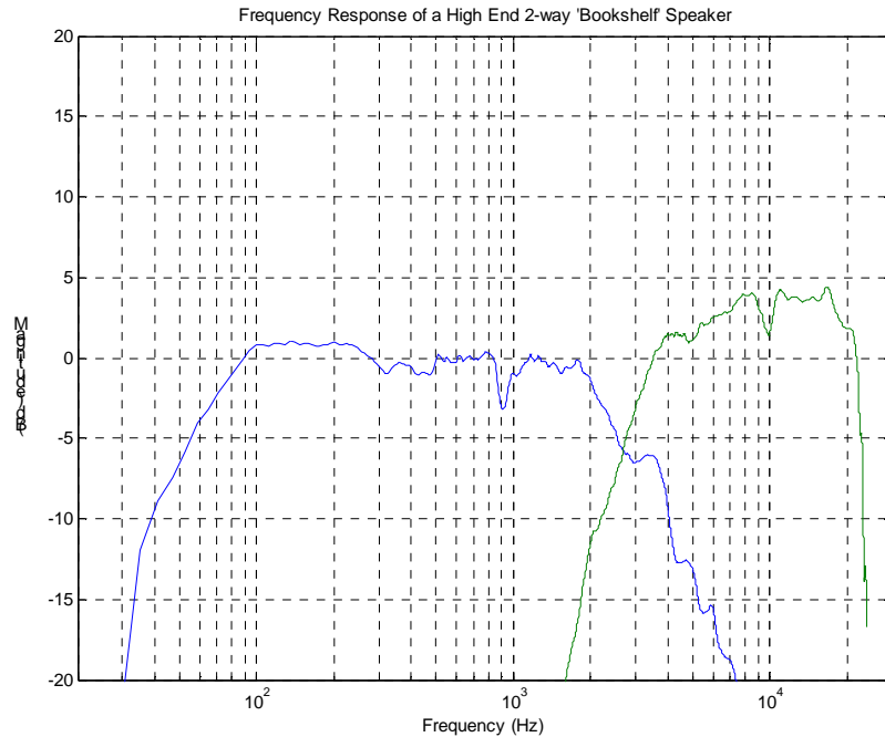
A typical frequency response of a two-way speaker system, showing both woofer and tweeter after passive crossovers. The sum of the woofer and tweeter across the crossover range (typically over two octaves) target a flat frequency-response on-axis.
